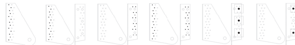
Wariant I BNF40, Wariant II BNG60, Wariant III BNG60, Wariant IV BNG60, Wariant V BNG60, Wariant VI BNG60
