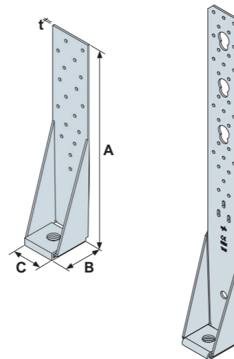
HTT4 / HTT5 HTT22E HTT31
