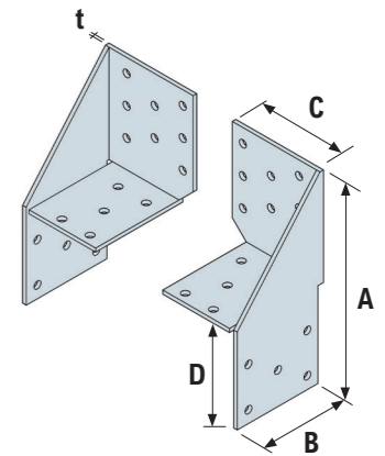
UNI130
