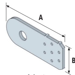
Adapter BNKK40/60
