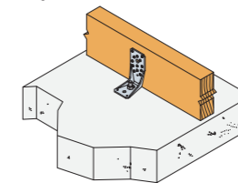
AKR95
